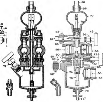
Figs. 3203-3204. "Bull's Eye" Locomotive Lubricator. Michigan Lubricator Co.
